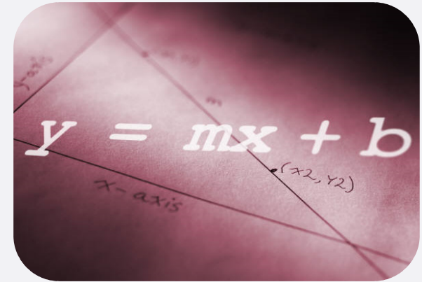
Customized Algorithms
